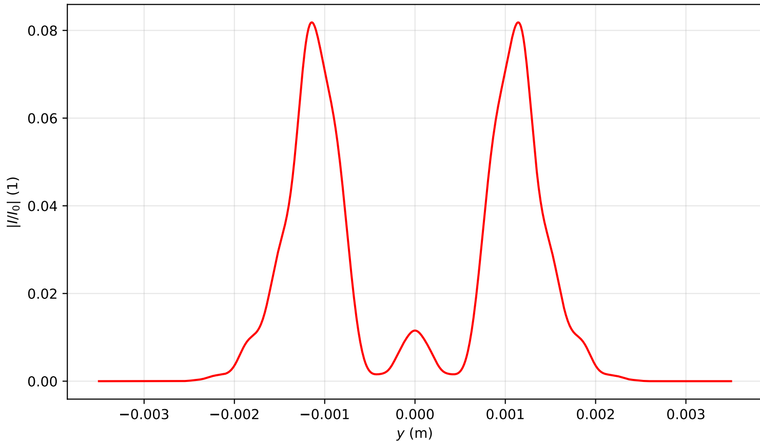
Intensity profile I(x=0, y, z=3.344)/I_0 , P_{in}=7.5P_{cr} , artificial time
